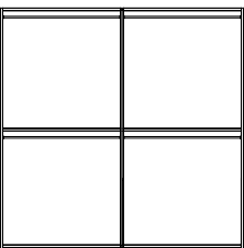
2/D SLIDING WARDROBE With 2 doors, 2 shelves and 4 hanging rods H226 - PJCVO040 inch W 90" D 27" H 89" cm L 228,7 P 68,2 H 226,3 Crts 9 kg 341 m 3 0,53 H239 - PJCVO020 inch W 90" D 27" H 94" cm L 228,7 P 62,8 H 239,1 Crts 9 kg 359 m 3 0,56
