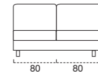
SCocca TERMINALE MAXI DX 182 Materasso-Mattress-Matelas 160 x 193 x 21
